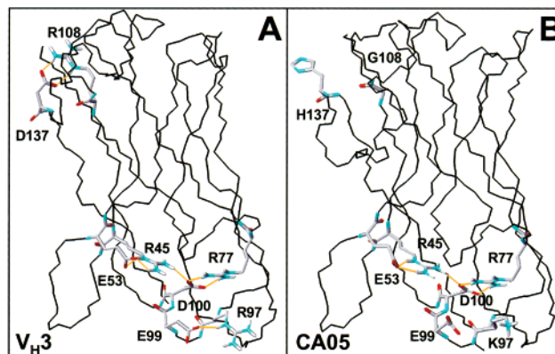
FIGURE 6: (A) V H3 domain of the KOL Fab fragment (PDB entry 2FB4) and (B) CA05 (PDB entry 1F2X) as an example for V HH fragments with residues colored by atom type which form putative salt bridges (orange). Images were generated using the program MOLMOL (26). Numbering scheme according to Honegger and Plückthun (5).
