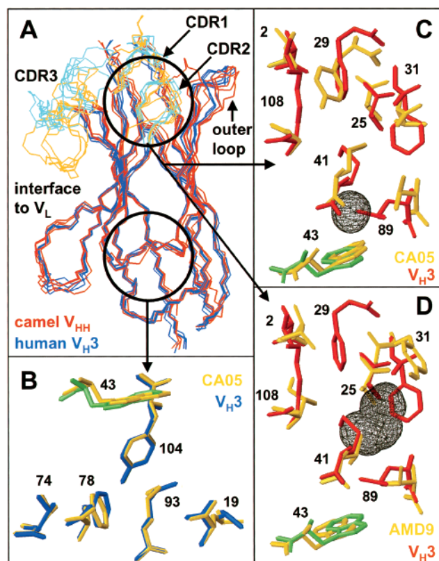
FIGURE 5: (A) Superposition of structures of V HH fragments (PDB entries 1HCV, 1BZQ, 1F2X, and 1KXQ) in red (CDRs in orange) and structures with human V H3 domains (PDB entries 1AQK, 1DEE, 1IGM, and 2FB4) in blue (CDRs in cyan). (B) Detailed view of the lower core. Superposition of CA05 (PDB entry 1F2X) in yellow and the V H3 domain of an anti-protein A Fab fragment (PDB entry 1DEE) in blue. The conserved Trp43 is shown in green. (C and D) Detailed view of the upper core. Superposition of CA05 (PDB entry 1F2X) (C) and of AMD9 (PDB entry 1KXQ) (D) in yellow with the V H3 domain of an anti-protein A Fab fragment (PDB entry 1DEE) in red. The conserved Trp43 is shown in green. The van der Waals contact surface was generated for a probe radius of 1.4 Å with the program MOLMOL (26). Cavities within the upper core of the V HH fragments are shown in black. Images were generated using the program MOLMOL (26). Numbering scheme according to Honegger and Plückthun (5).
